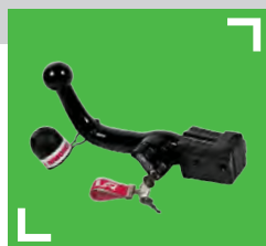
MODEL M manually detachable ball with safety lock
